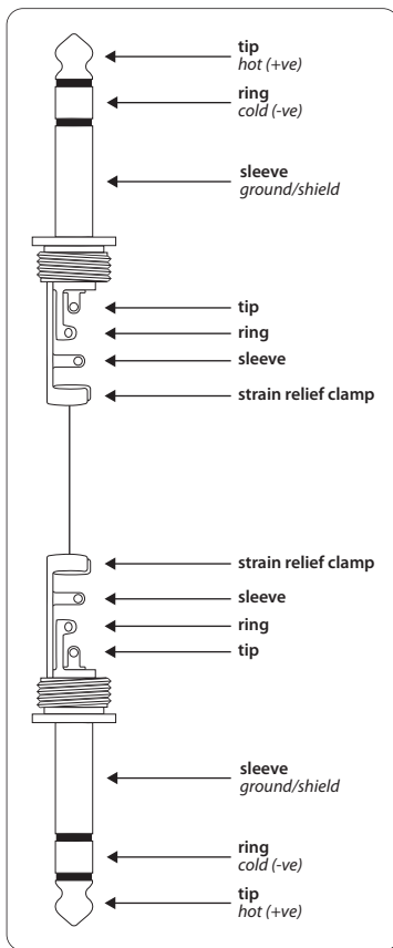
Fig. 4.2: Patch cord with balanced, \frac{1}{4} " TRS plugs
