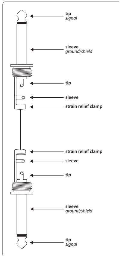
Fig. 4.1: Patch cord with unbalanced, \frac{1}{4} " TS plugs
